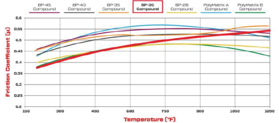
BP-30 Friction Coefficient and Temperature Values
